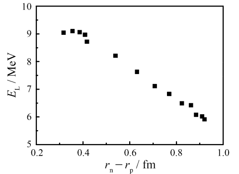
Fig. 3 The centroid energies of the isovector dipole strengths in the low-lying region below 10 MeV versus the differences of the neutron and proton rms radii in Ni-isotopes.
