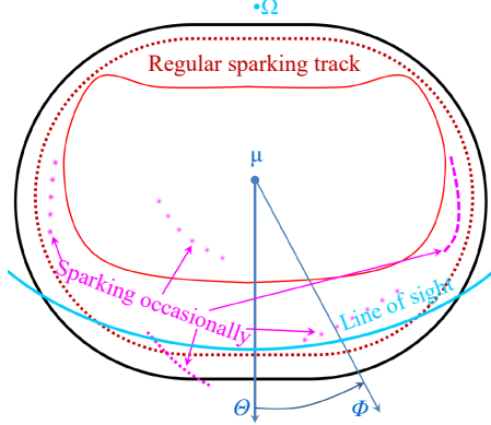
Fig. 3 (color online) The magnetic pole of a pulsar in spherical coordinates with polar angle \Theta and azimuthal angle \Phi , where \mu symbolizes the magnetic pole and \Omega the spin axis. Regular sparking occurs along the “regular track”. However, if intercepted by a small hill, occasionally, there may be preferential point discharge, observed as a different type of sparking, and this could suppress regular sparks.
